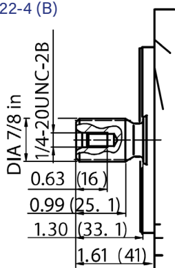
S Splined shaft 7/8 in in 13T 16/32 DP SAE J744-22-4 (B)
