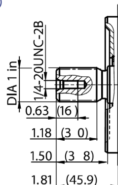
U Splined shaft 1 in 15T 2) 16/32 DP SAE J744-25- 4 (B-B)
