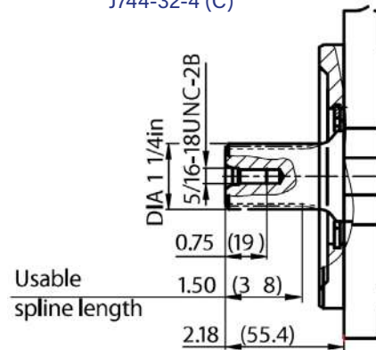
R Splined shaft 1 1/4 in 14T 12/24 DP SAE J744-32-4 (C)
