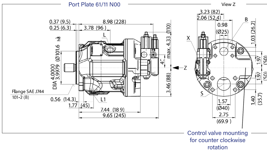
Port Plate 61/11 N00
