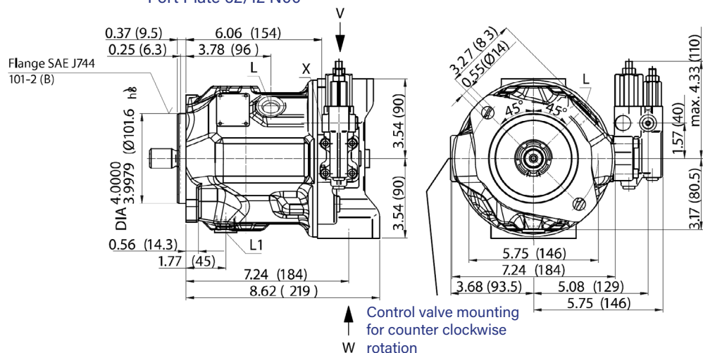
Port Plate 62/12 N00
