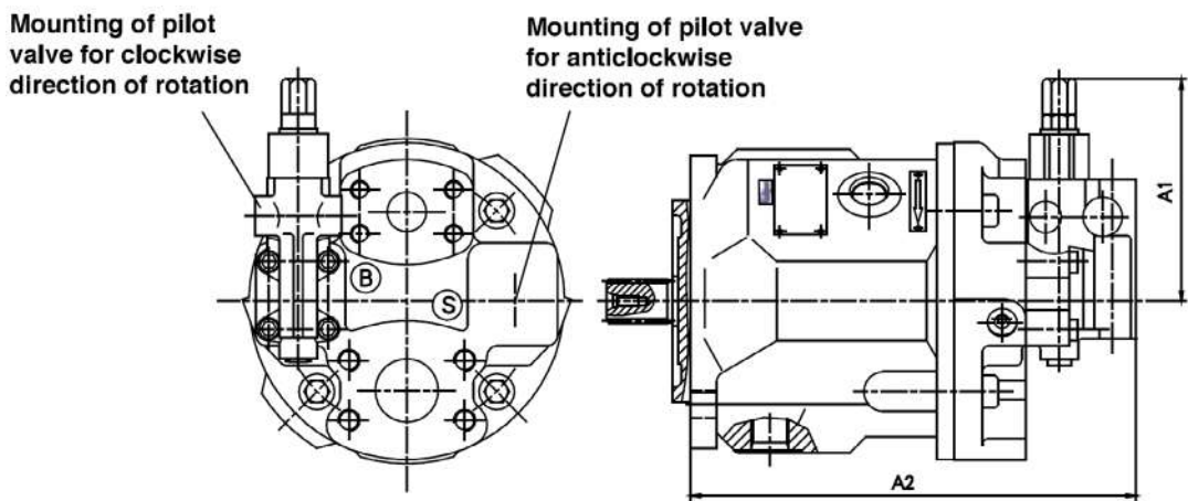
Service Ports at Rear; Models 62N00 and 12N00
