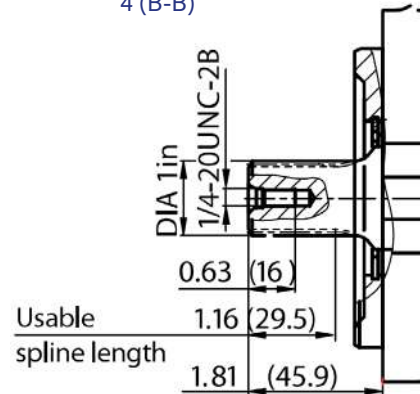
R Splined shaft 1 in 15T 16/32 DP SAE J744-25- 4 (B-B)
