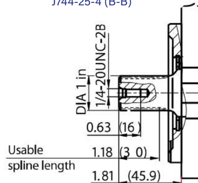
W Splined shaft 1 in 2) 15T 16/32 DP SAE J744-25-4 (B-B)
