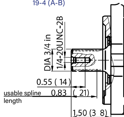
W Splined shaft 3/4 in 11T 16/32 DP SAE J744- 19-4 (A-B)
