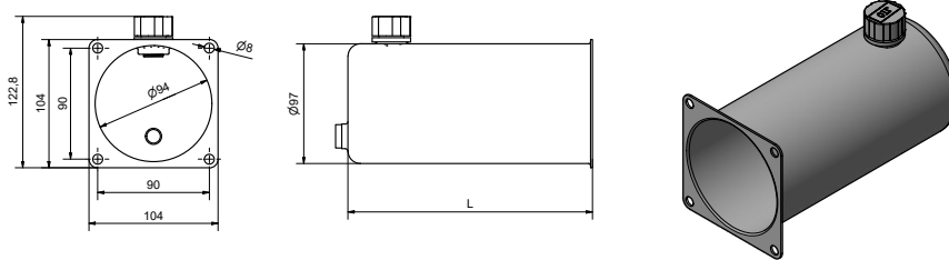
METALLIC TANK RECTANGULAR BASE GROUP K0
